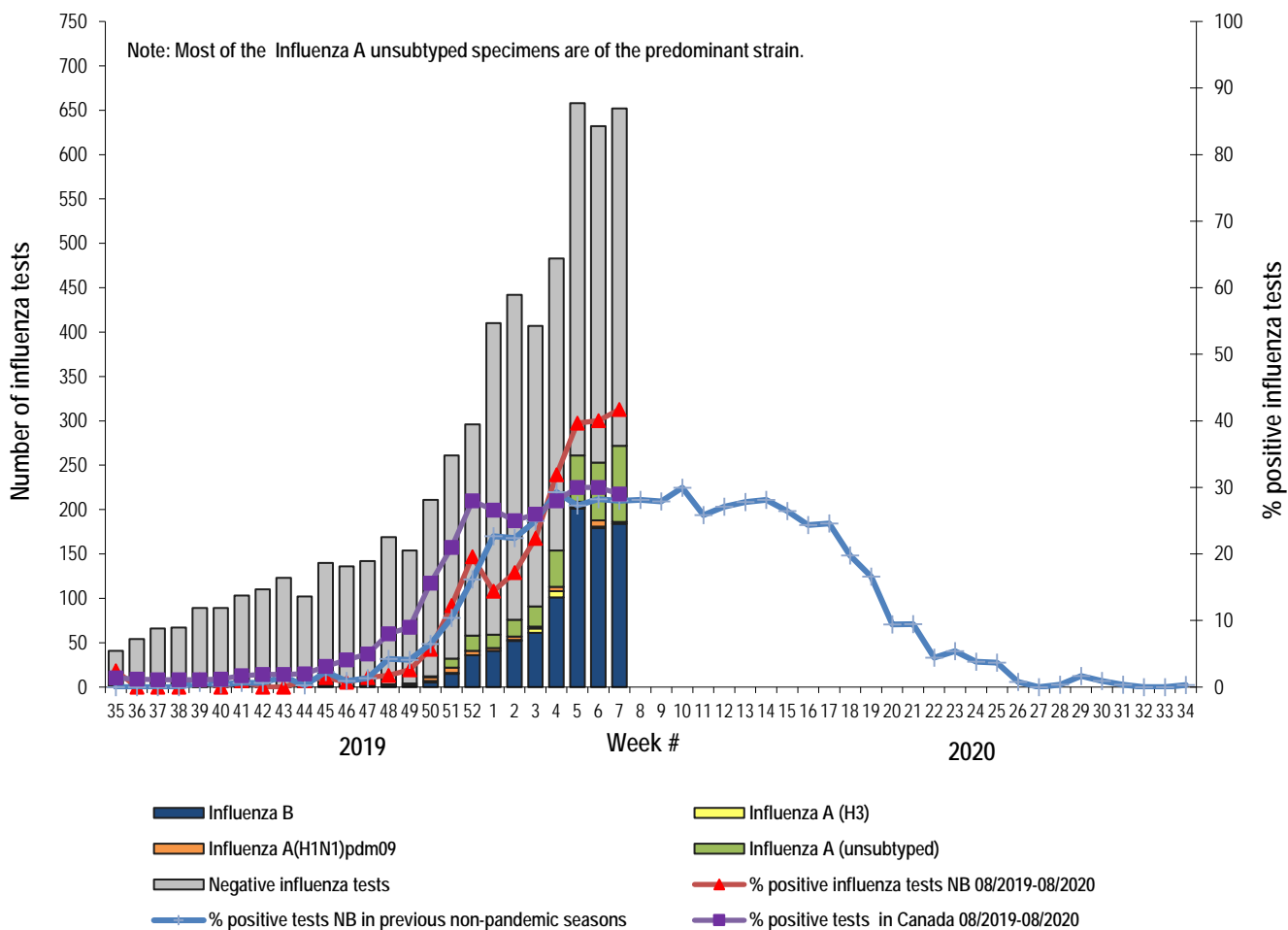
Graph 1: Number and percent of positive influenza specimens 2 in New Brunswick by week, up to February 15, 2020 (data source: G. Dumont Lab results)
